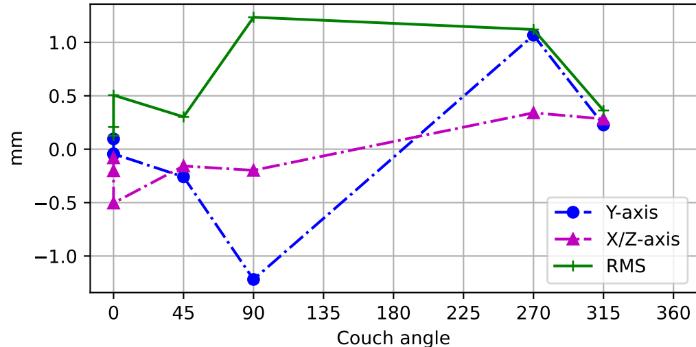
Collimator wobble
