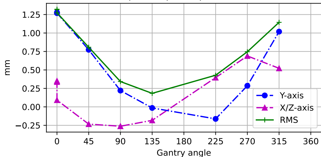
In-plane Couch displacement
