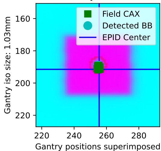
Gantry wobble
