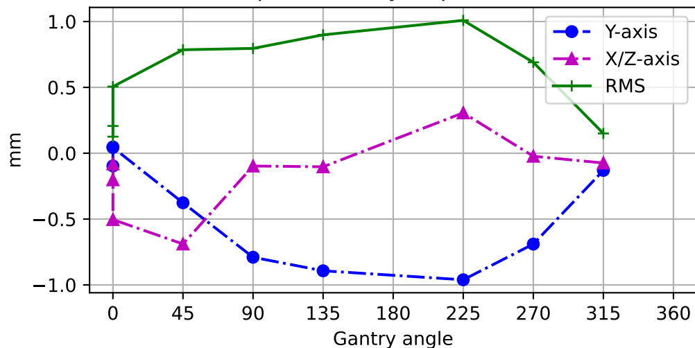
In-plane Collimator displacement
