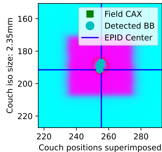
Couch wobble
