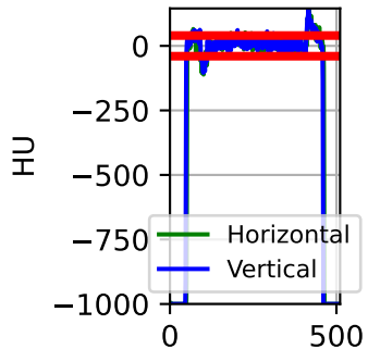
Uniformity Profile
