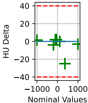
HU linearity
