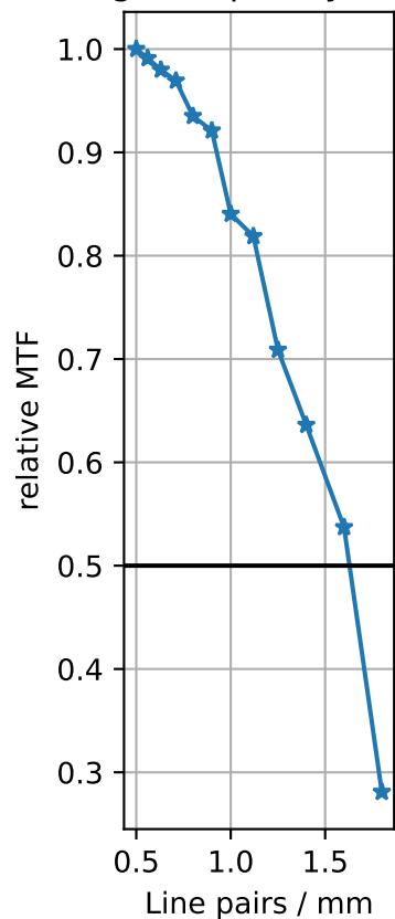
High-frequency rMT
