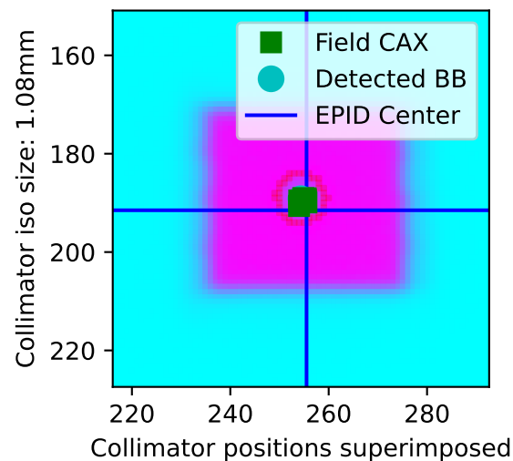
Collimator wobble
