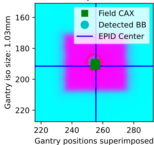
Gantry wobble
