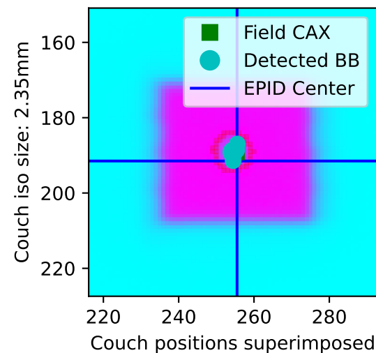
Couch wobble
