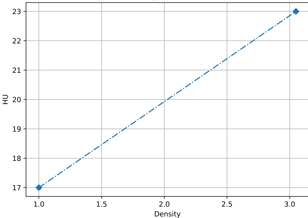
Density vs HU curve
