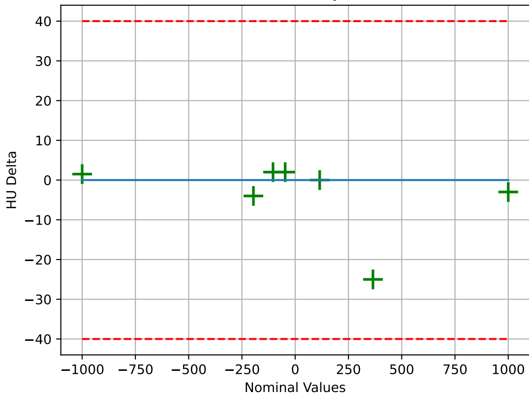
HU linearity
